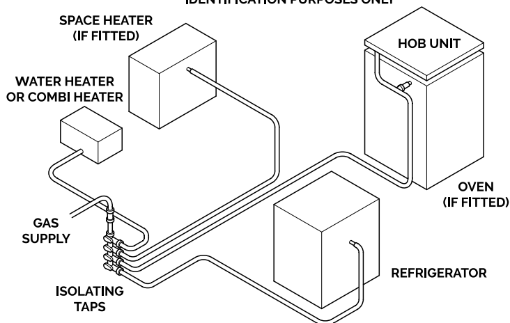
GAS SYSTEM SCHEMATIC DIAGRAM FOR ONLY IDENTIFICATION PURPOSES ONLY
