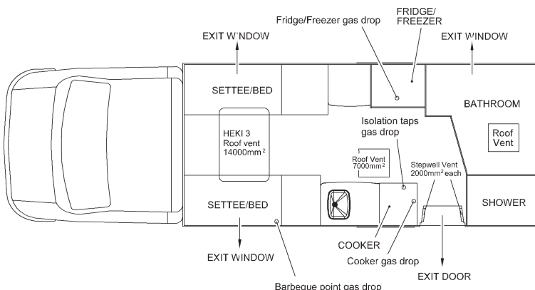
Cotswold EB Ventilation Diagram
