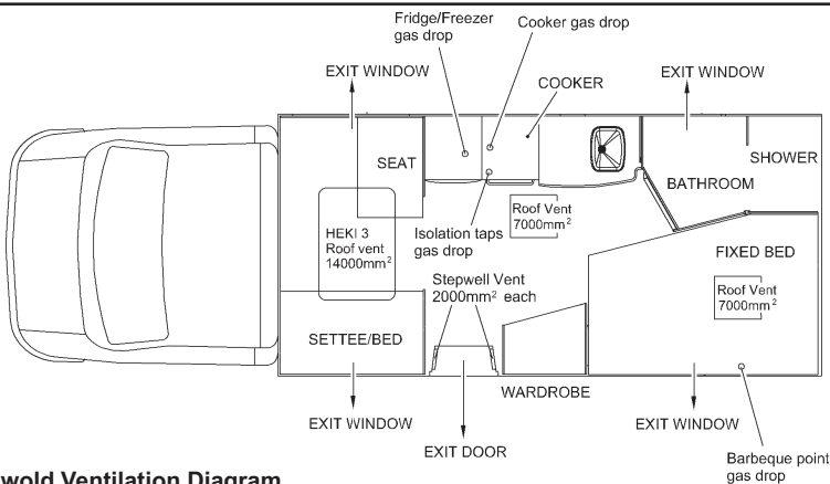
Cotswold Ventilation Diagram
