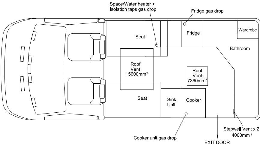
Broadway EB Ventilation Diagram
