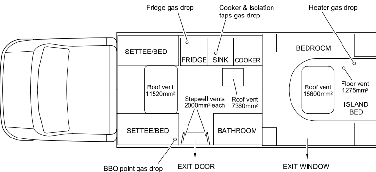
Corinium RB Ventilation Diagram
