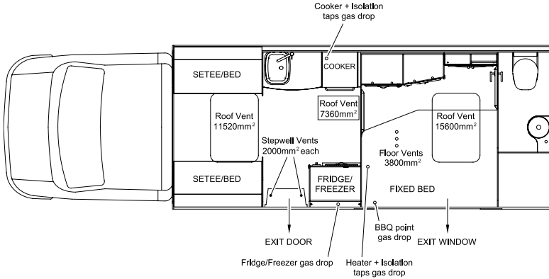
Corinium FB Ventilation Diagram
