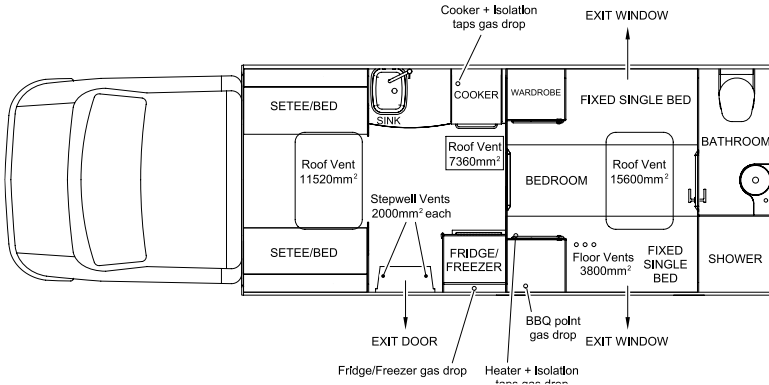
Corinium Duo Ventilation Diagram
